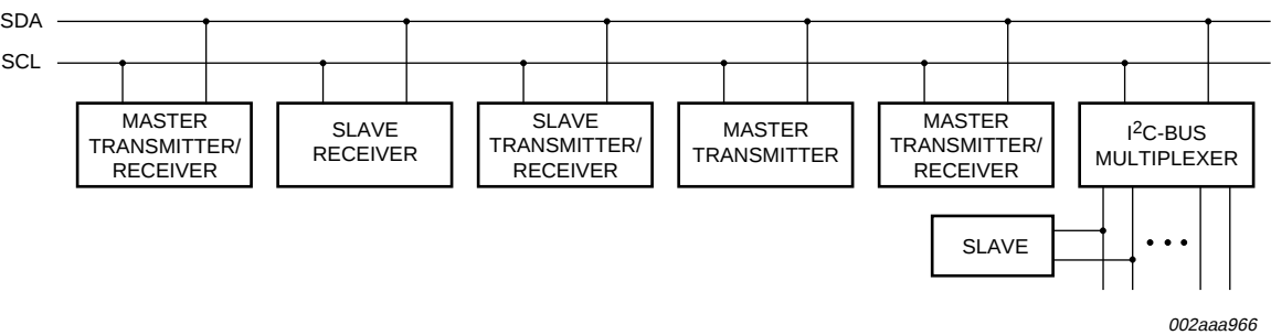
Fig 20. System configuration
